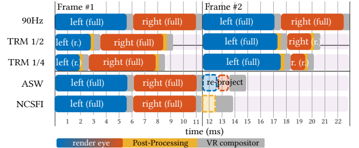
Fig. 14. Measured performance of 90Hz full resolution rendering on HTC Vive for two consecutive frames averaged over 1500 samples (top); compared with our TRM method with 1/2 and 1/4 resolution reduction (center and bottom). Dashed lines (Frame 2 for ASW and NCSFI) indicate estimated time duration. Unutilized time periods can be used to load or compute additional visual effects or geometry.
