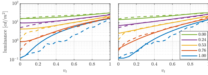
Fig. 9. Dashed lines: measured display luminance for red primaries ( v_t ), given a range of different v_{t-1} pixel values (line colors). Solid lines: predicted values without temporal display model (left) and with our temporal model (right).
